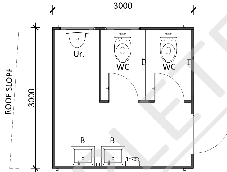
FLOOR PLAN
