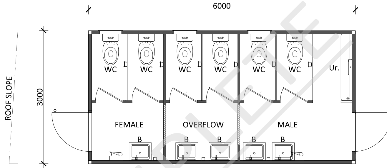
- FLOOR PLAN
