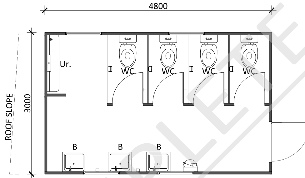
— FLOOR PLAN
