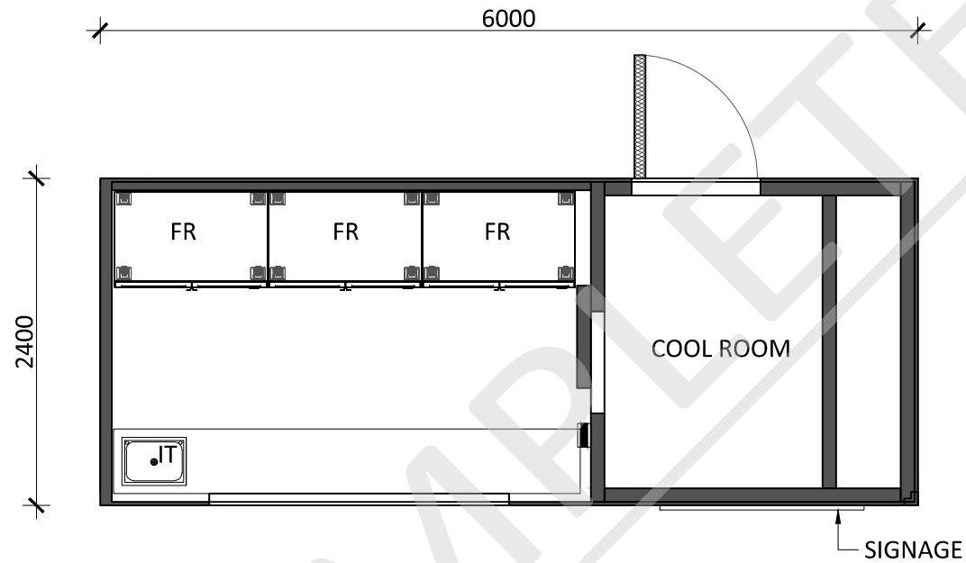
— FLOOR PLAN
