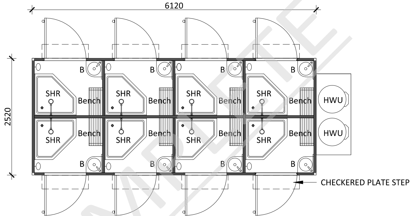
- FLOOR PLAN
